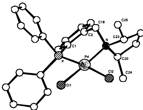
Figure 1. Crystal structure of the Pd dichloride complex 13 . Selected distances (Å) and angles (°): Pd–N 2.138(3), Pd–P 2.237(1), Pd–Cl1 2.286(1), Pd–Cl2 2.370(1), P–Pd–N 92.5(1), Cl1–Pd–Cl2 86.51(4), P–Pd–Cl1 86.21(4), N–Pd–Cl2 94.8(1)
