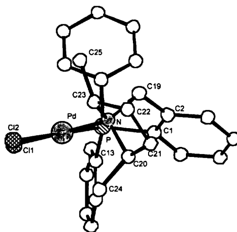
Figure 2. X-Ray crystal structure (side view) highlighting the pyrrolidine ring conformation and the positions of the C24 and C25 methyl groups
